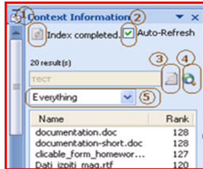
Figure 4. Screenshot from the context-aware ‘live’ search agent’s user interface: 1. Indexing button. 2. Change behaviour button. 3. Search the Desktop button. 4. Search the Web button. 5. Filters list.
