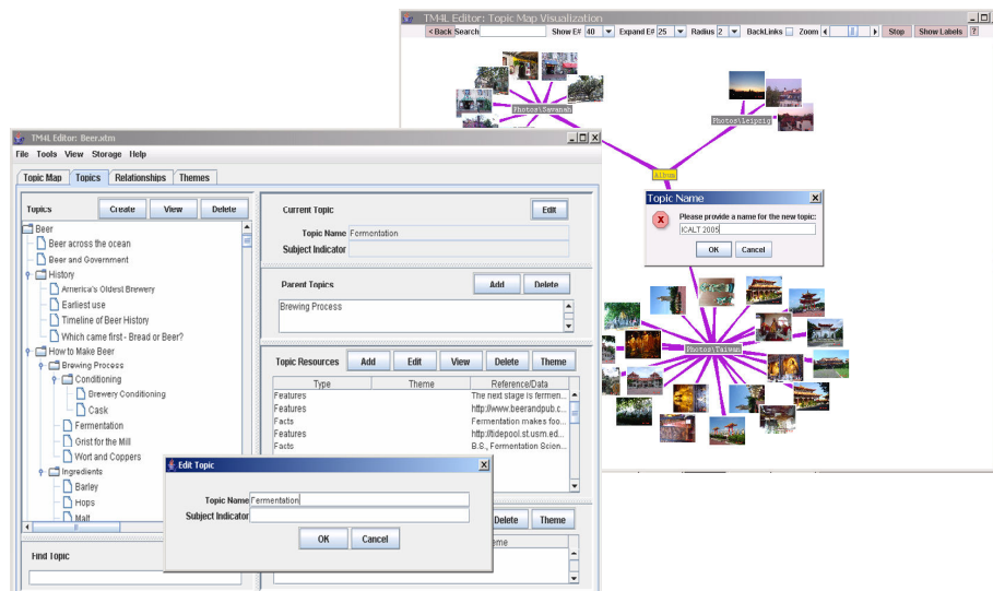
Figure 3. Screenshots from the TM4L Editor: Textual and Visual Topic editing.
